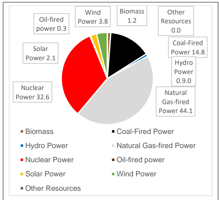
Exhibit B: Source of Electricity Supplied for the 12 months ending 12/31/2024
